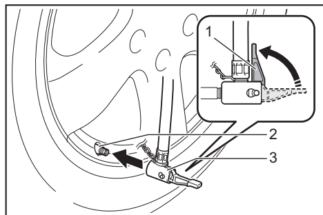
► 1. Air chuck clamp 2. Valve stem 3. Air chuck
